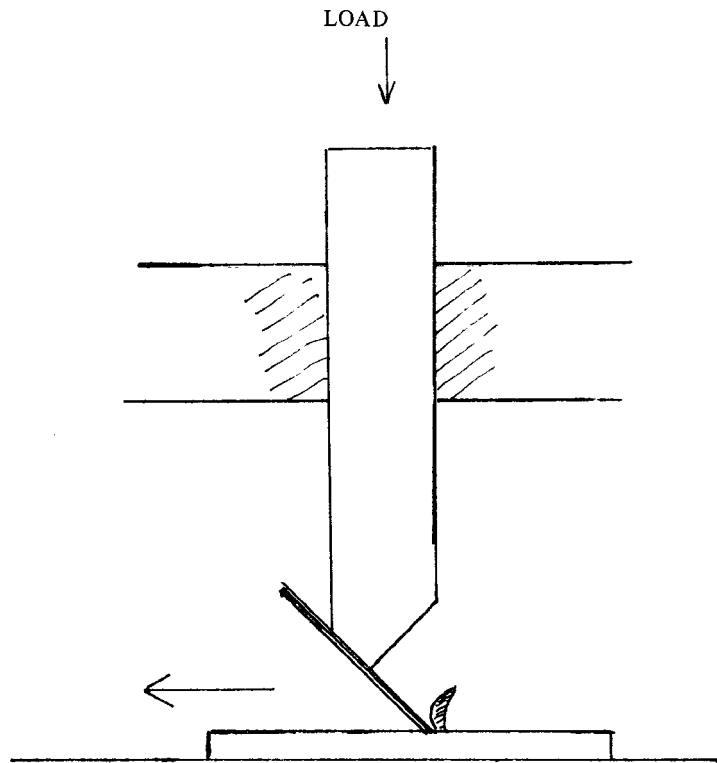
Fig. 1.1 Rossman Chisel Adhesion Test.
